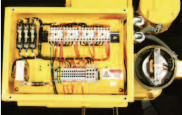
Basic Control Box and Motor Brake
